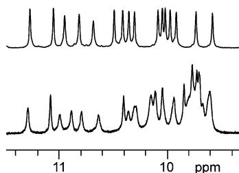
Figure 6. Part of the 700 MHz ^1\text{H} NMR spectra of 20mer 10 (top) in \text{CDCl}_3 and of 40mer 11 (bottom) in \text{CD}_2\text{Cl}_2 showing aryl-CONH-aryl resonances.
