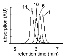
Figure 5. Overlay of the SEC traces of pentamer 1 , decamer 6 , 20mer 10 , and 40mer 11 on a TSK-GEL SUPER HM-M column. Conditions of separation compatible with the very low solubility of 11 were found using a \text{CHCl}_3/\text{pyridine} mixture (85:15 vol/vol) at 40 °C. Detection was carried out at 350 nm.
